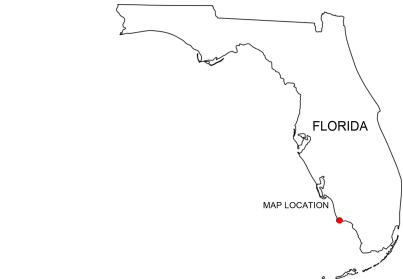
Tsunami Sources Modeled for the Marco Island coastline
